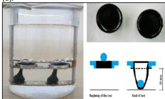
Figure .14: Softening point test.
